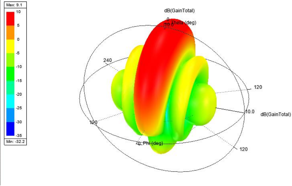
Gain Plot 3
