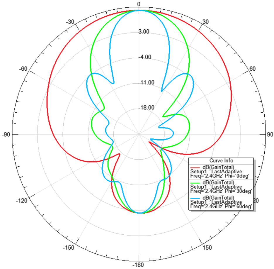
Gain Plot 3
